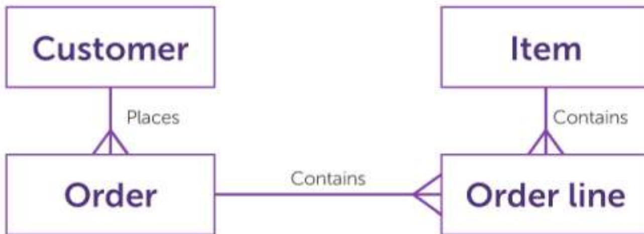
A simple E-R diagram for an online ordering system
