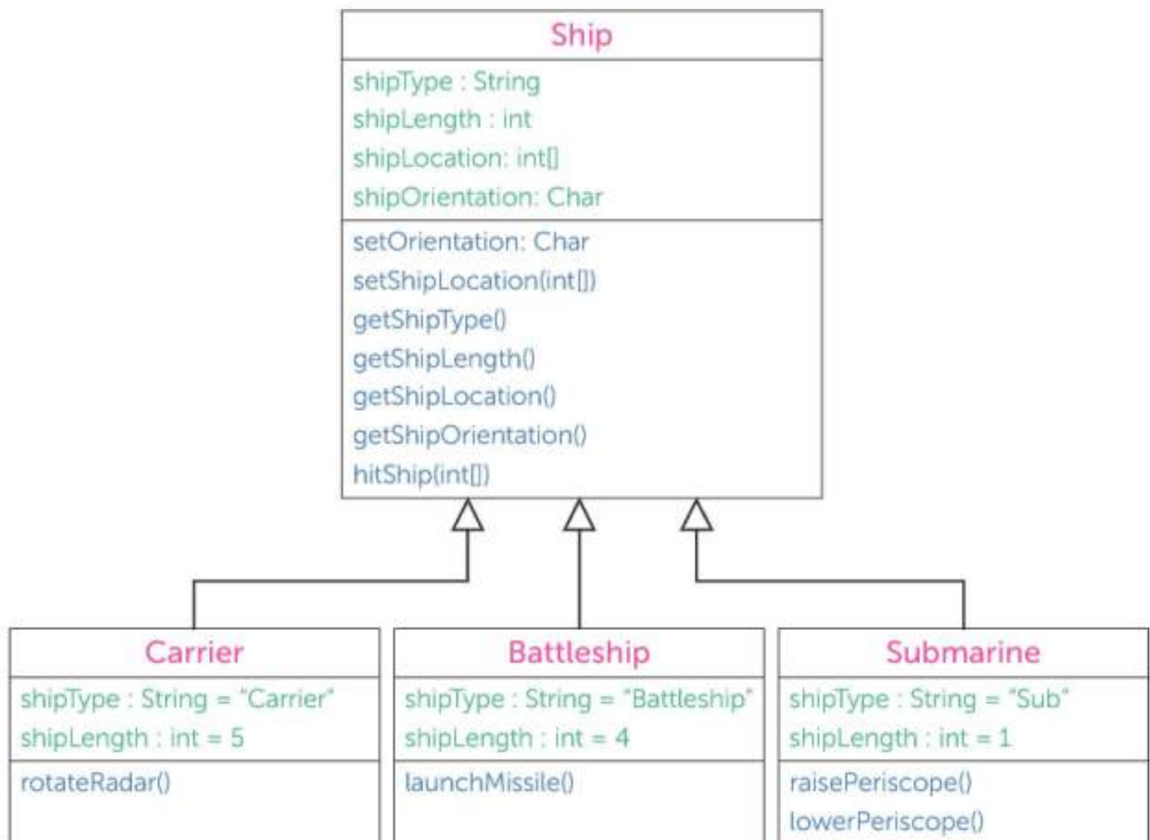
Three subclasses of the Ship class showing inheritance
