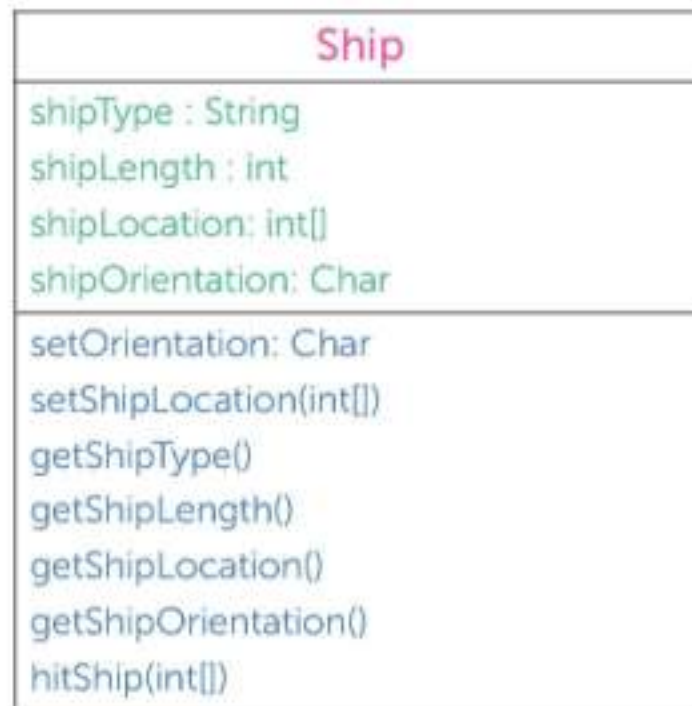
An example of one class
